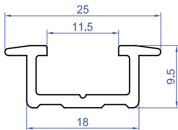
Recessed Bottom Track (7014)
