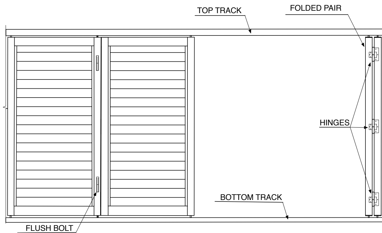
FRONT VIEW
