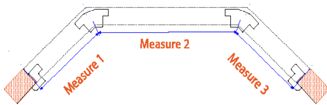
Corner Window: Inside Mount (L or Z)
