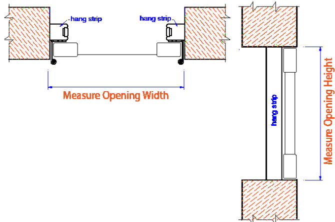
Hinged No Frame: L Hinge and Hang Strip
