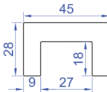
TOP CHANNEL (4050)
