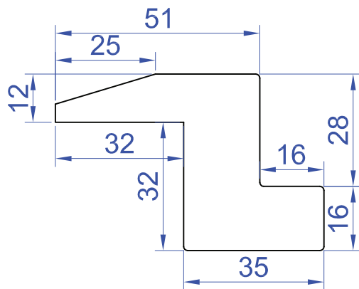
4021 Bevelled Z
