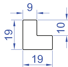
SIDE CHANNEL (4052)
