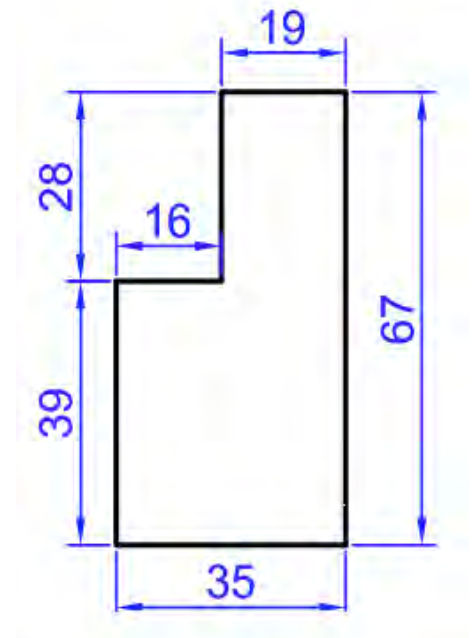
FLAT 67MM (4034)
