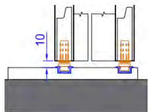
Recessed Track
