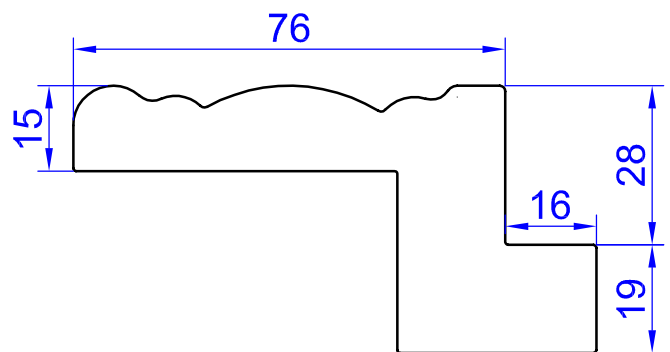
Z CROWN (4009)
