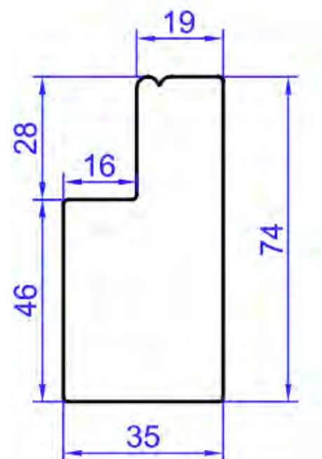
BEADED 74MM (4037)
