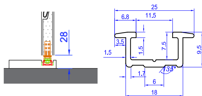
Recessed Track
